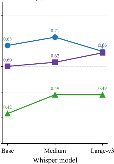
(b) One-shot
