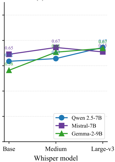
(c) Few-shot
