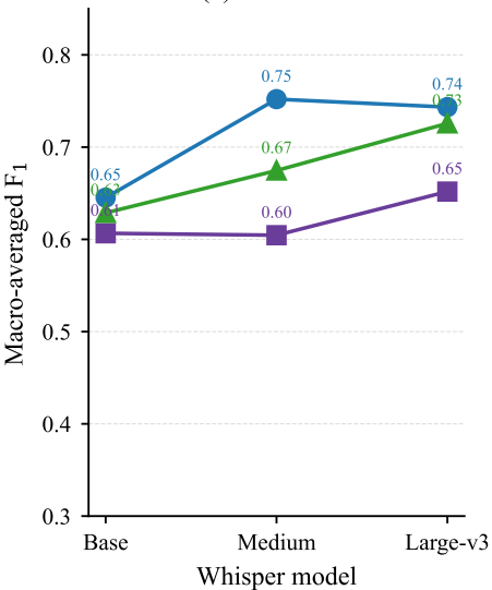
(a) Zero-shot
