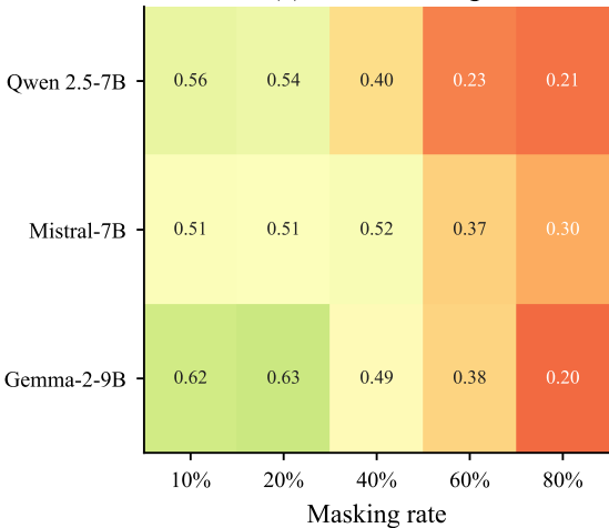
(a) Word masking
