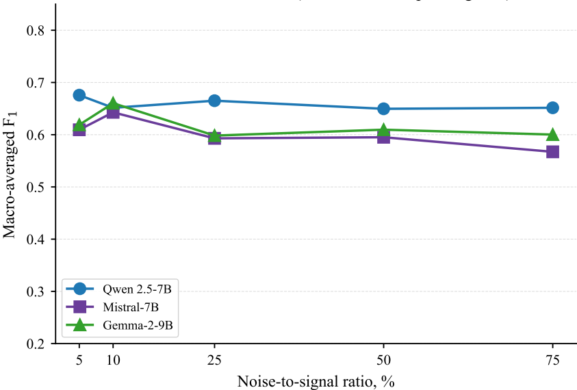
Audio noise robustness (zero-shot, Whisper-large-v3)
