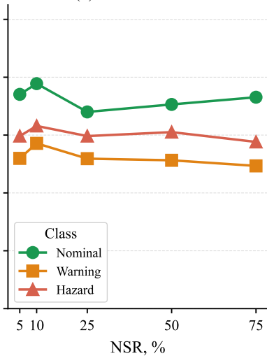
(c) Gemma-2-9B
