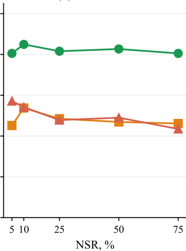
(b) Mistral-7B
