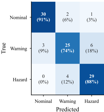
(a) Confusion matrix
