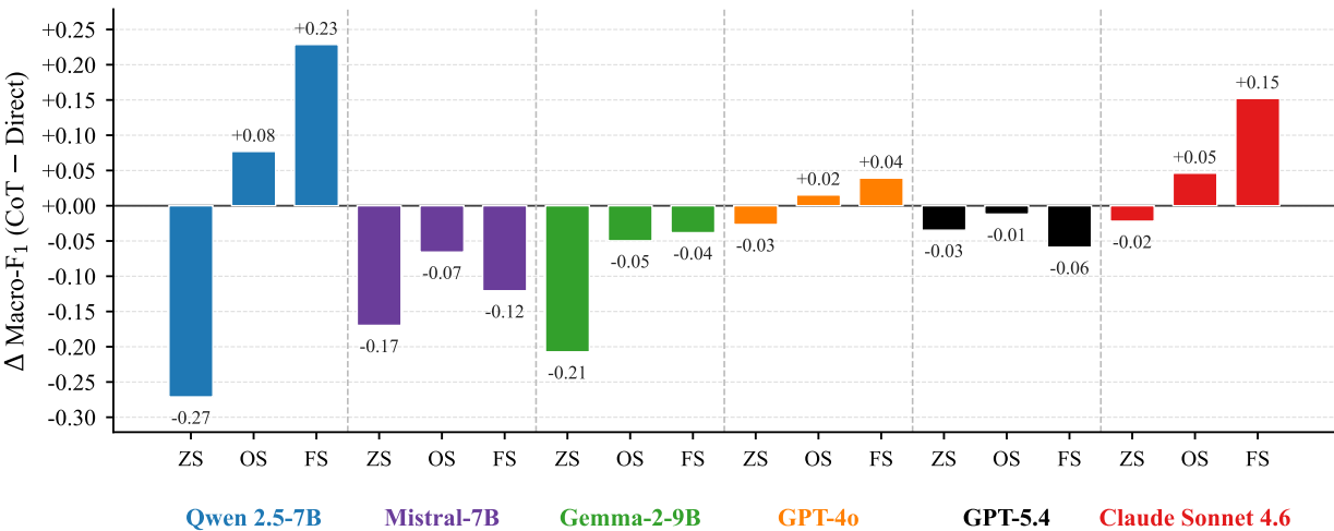
Effect of chain-of-thought on F 1
