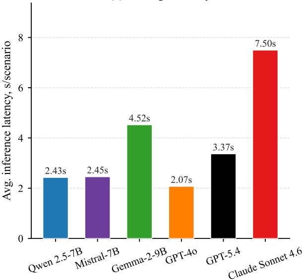
(a) Average latency
