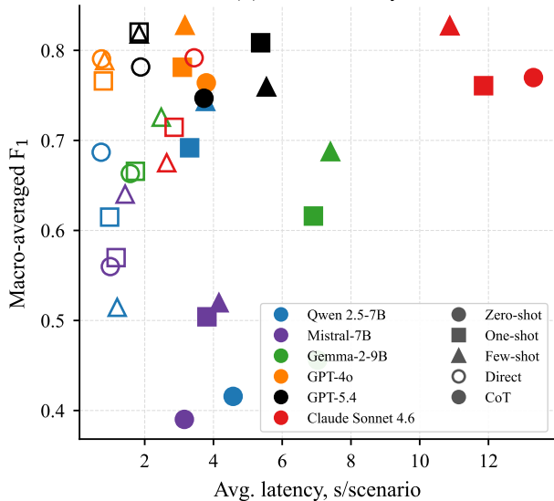
(b) F_1 vs. latency
