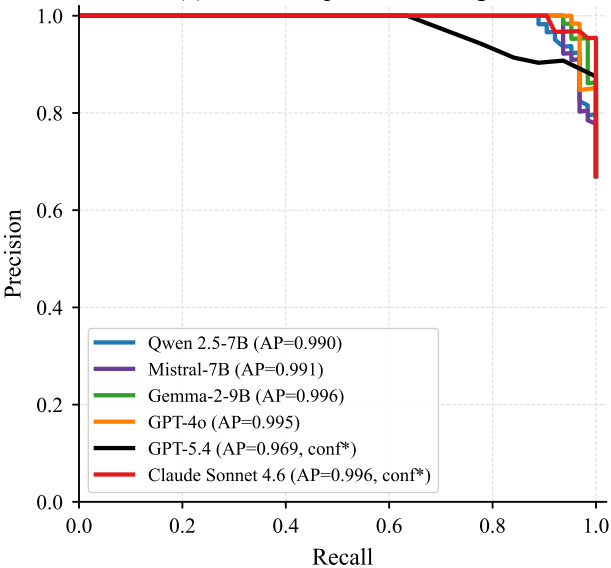
(a) PR curve, positive = danger
