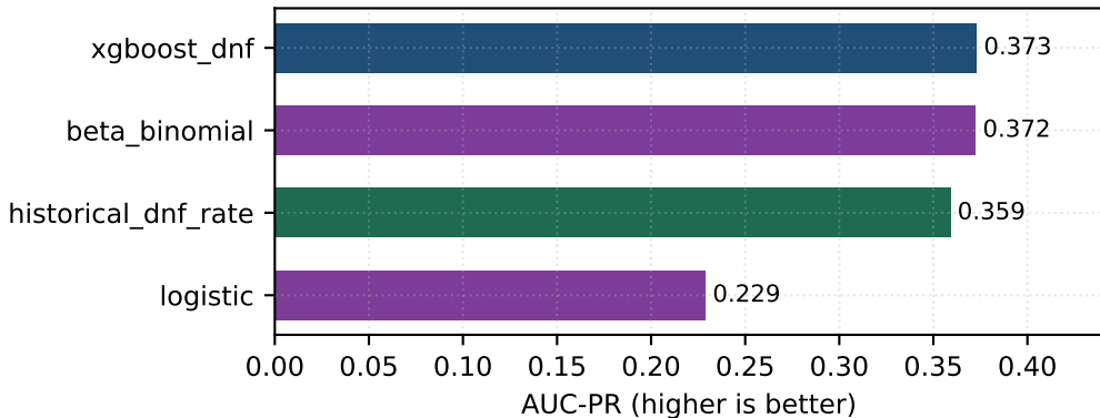
T3 DNF prediction: AUC-PR by baseline
