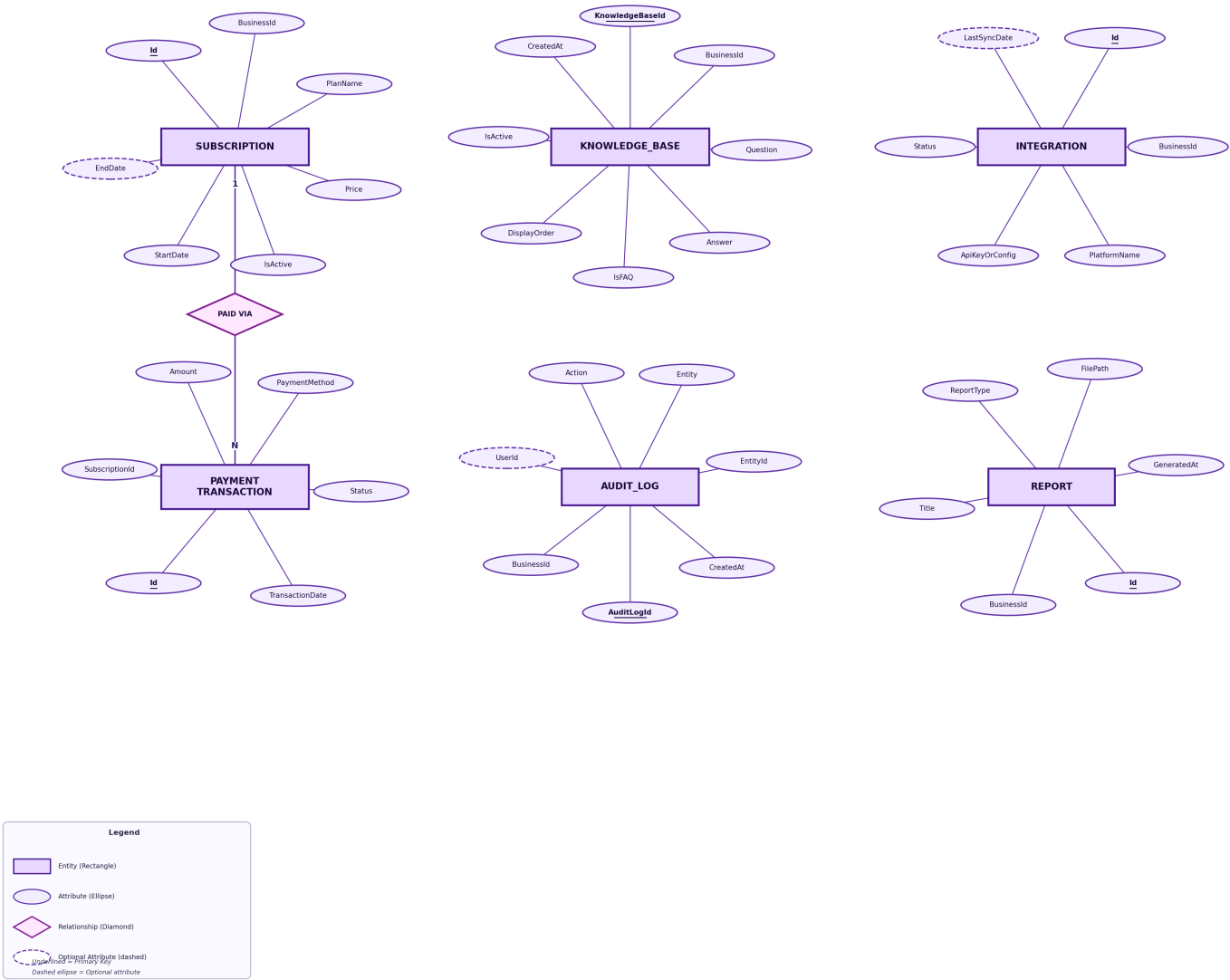
Chen ERD — Business Management Domain
