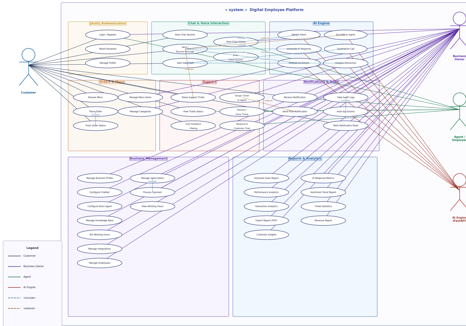
UML Use Case Diagram — Full System
