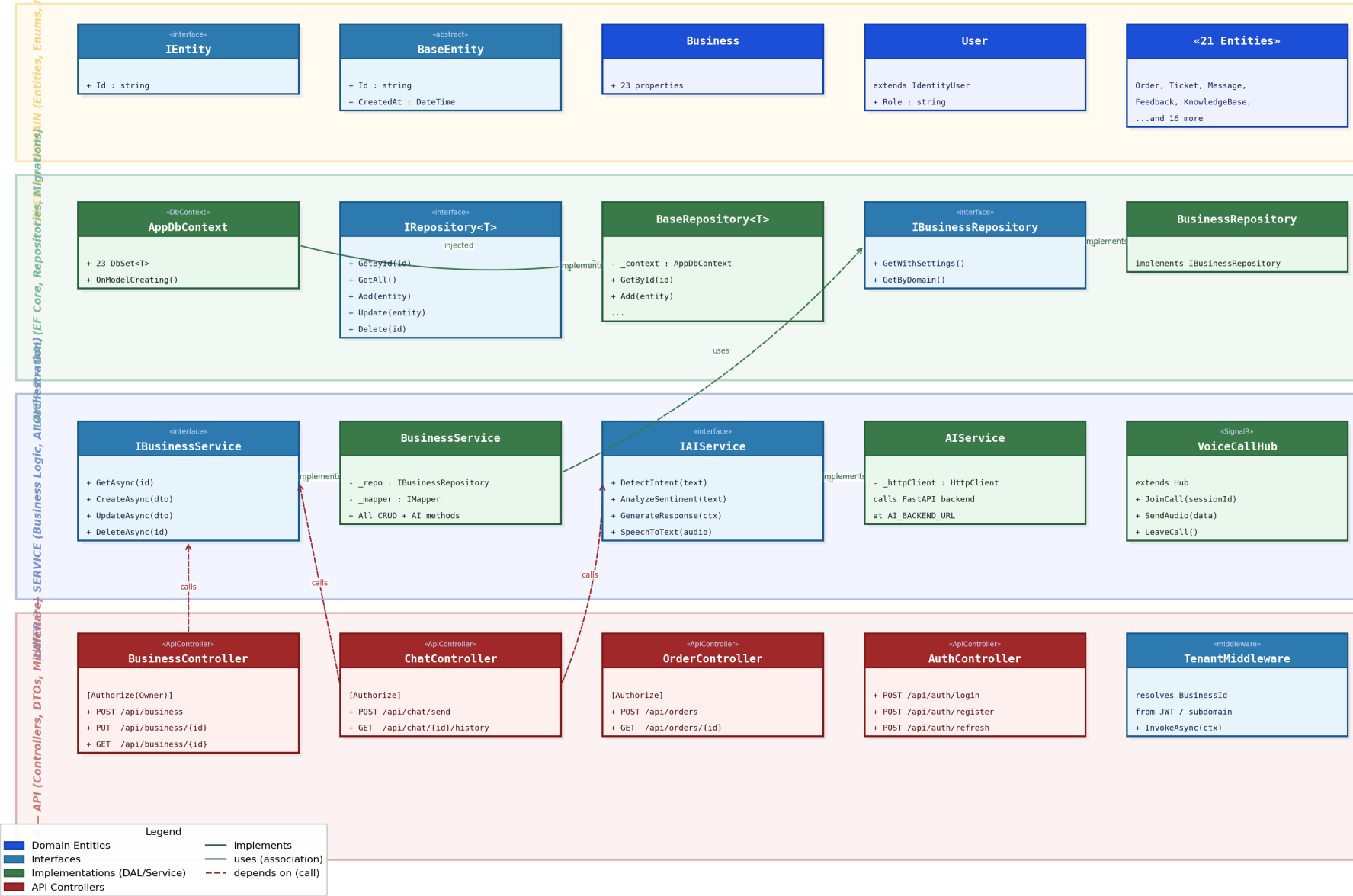
Class Diagram — Architecture Overview (Clean Architecture layers)
