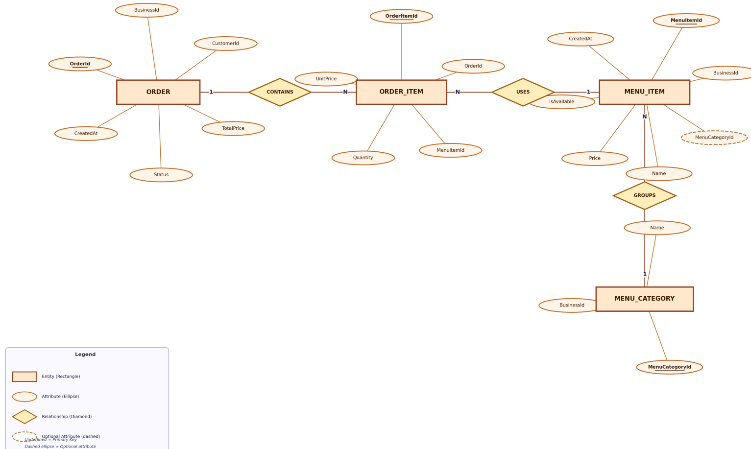
Chen ERD — Orders & Menu Domain
