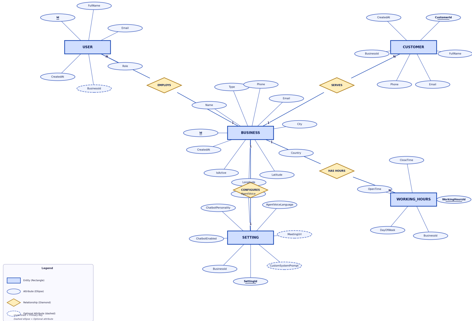
Chen ERD — Core Domain
