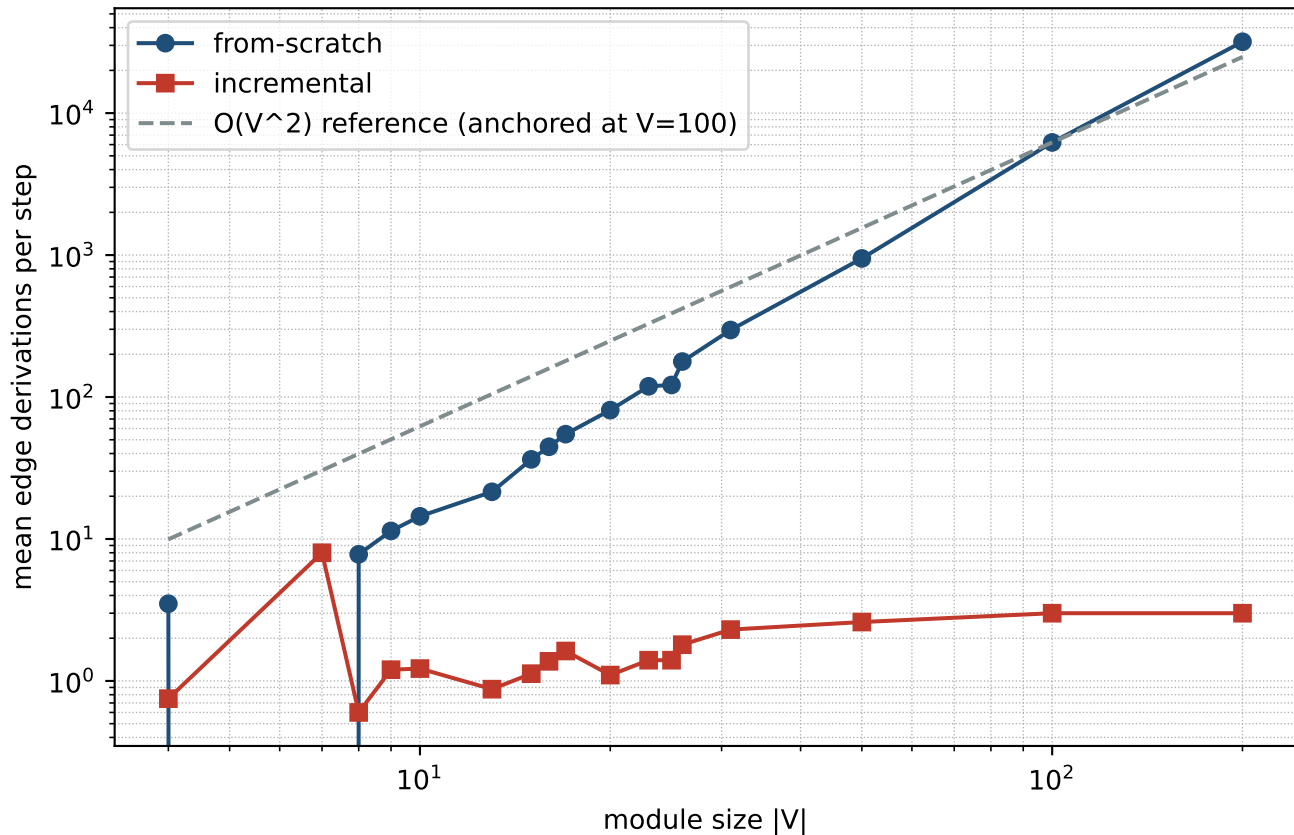
Smell-dependency graph maintenance: from-scratch vs. incremental
