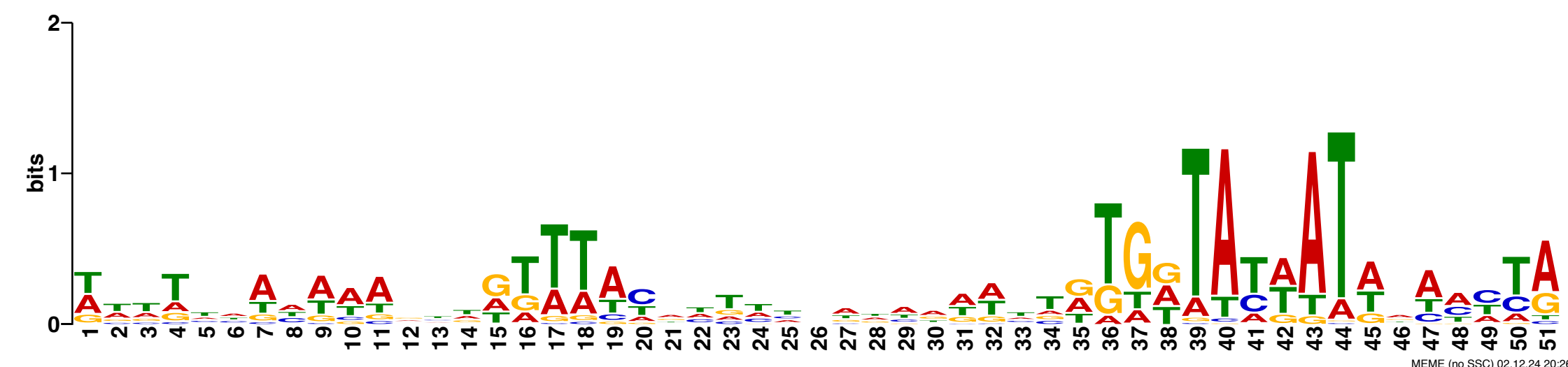
T4 early promoters
