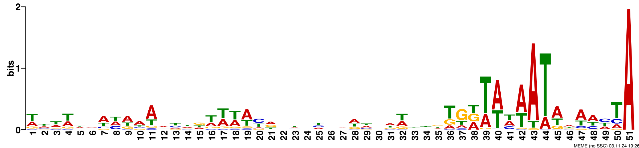
T4 +1A promoters
