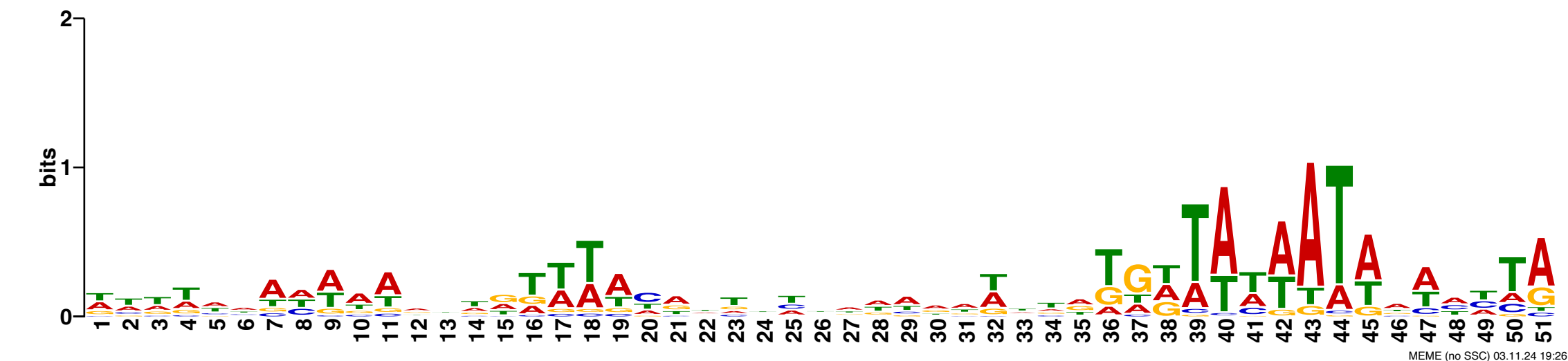
T4 primary promoters
