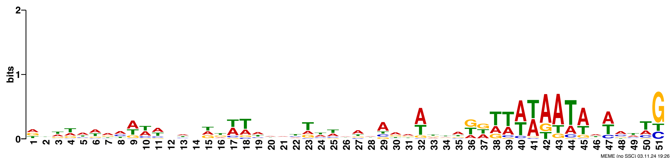
T4 all non +1A promoters
