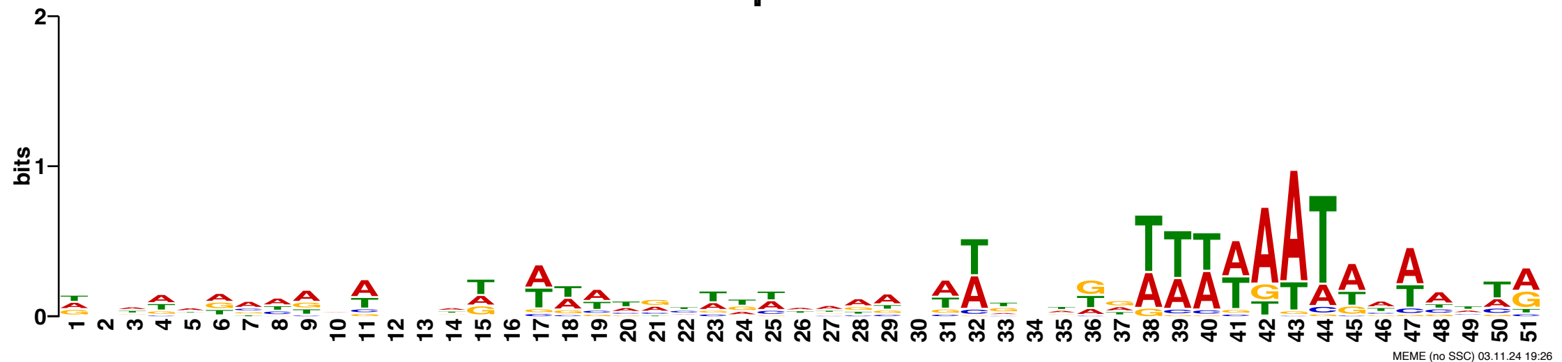
T4 internal promoters
