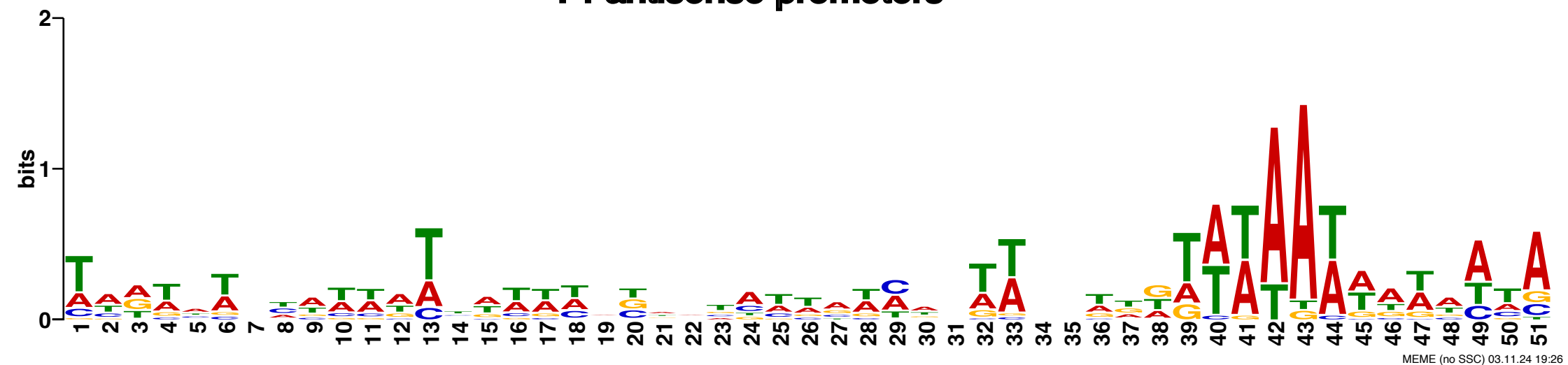
T4 antisense promoters
