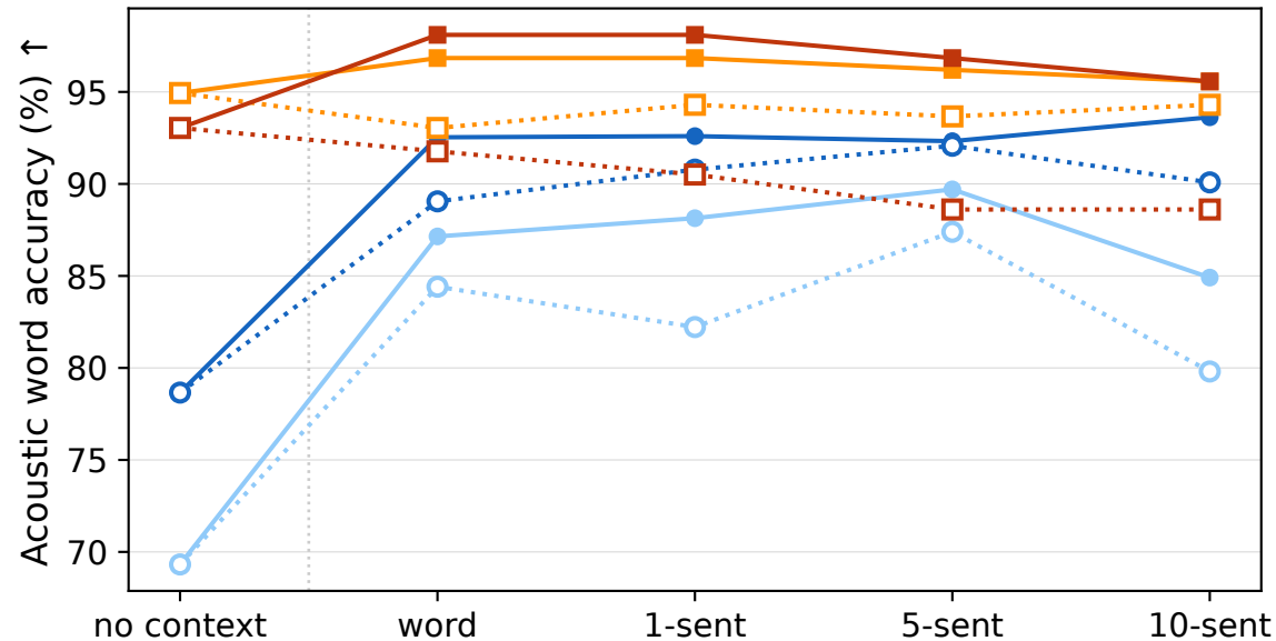
Qwen2.5-Omni-7B
