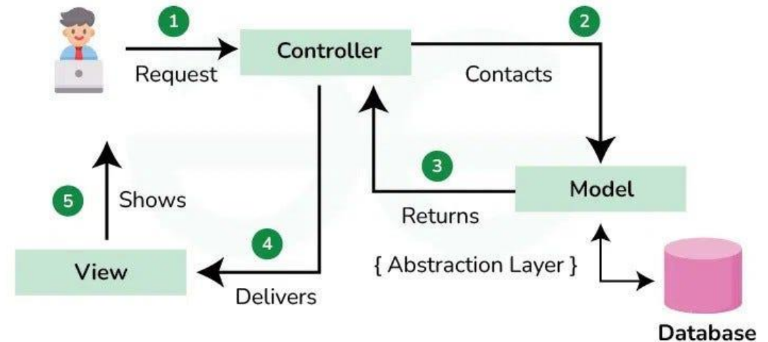
MVC Design Pattern
