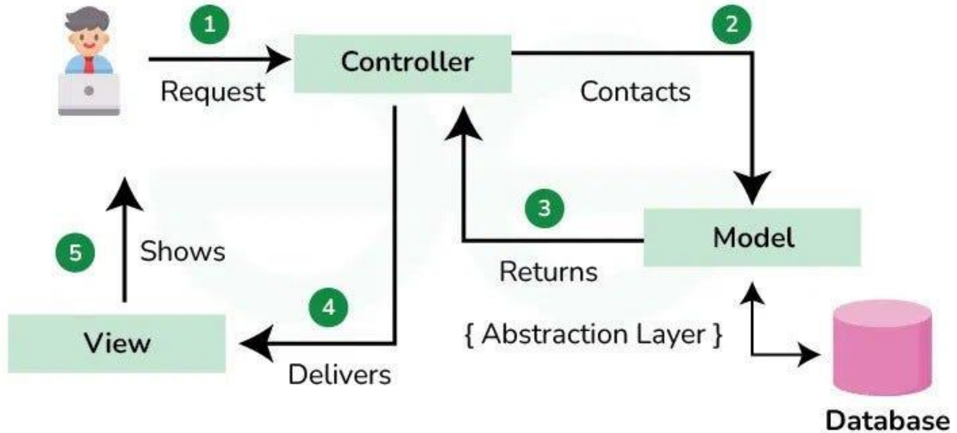
MVC Design Pattern
