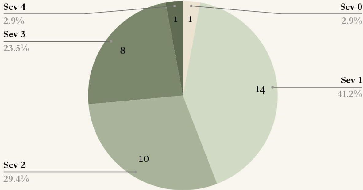
Severity Breakdown
