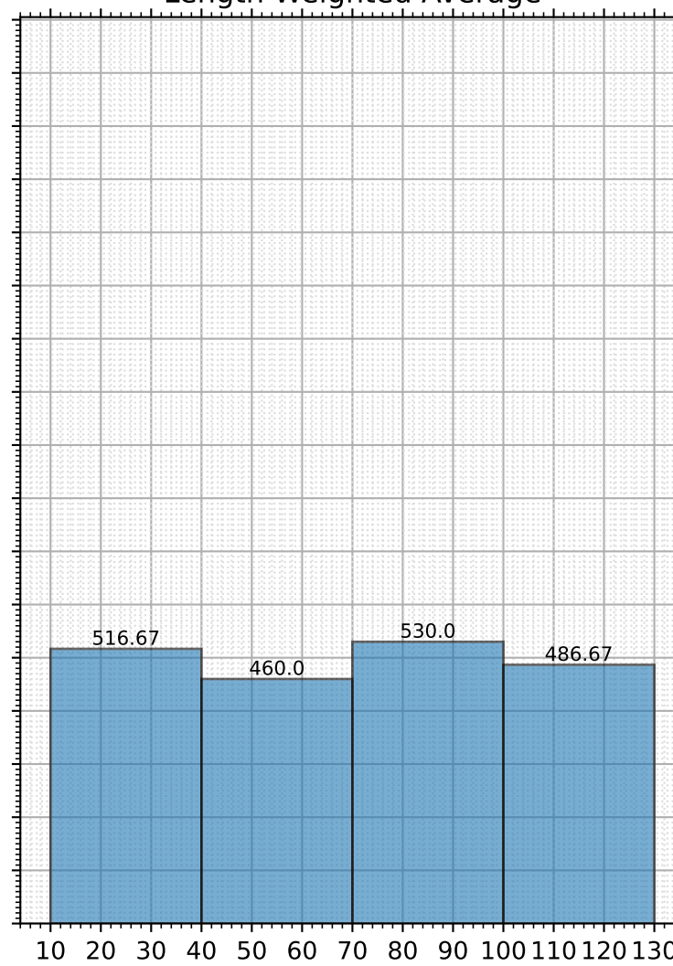
Average
