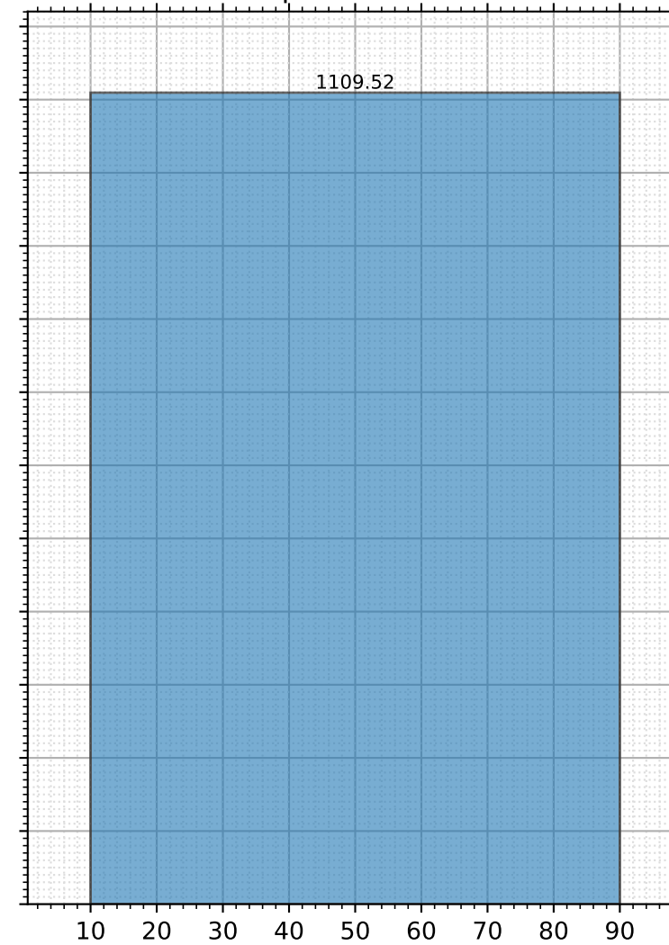
ProportionalSum
