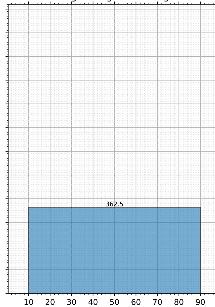
Average
