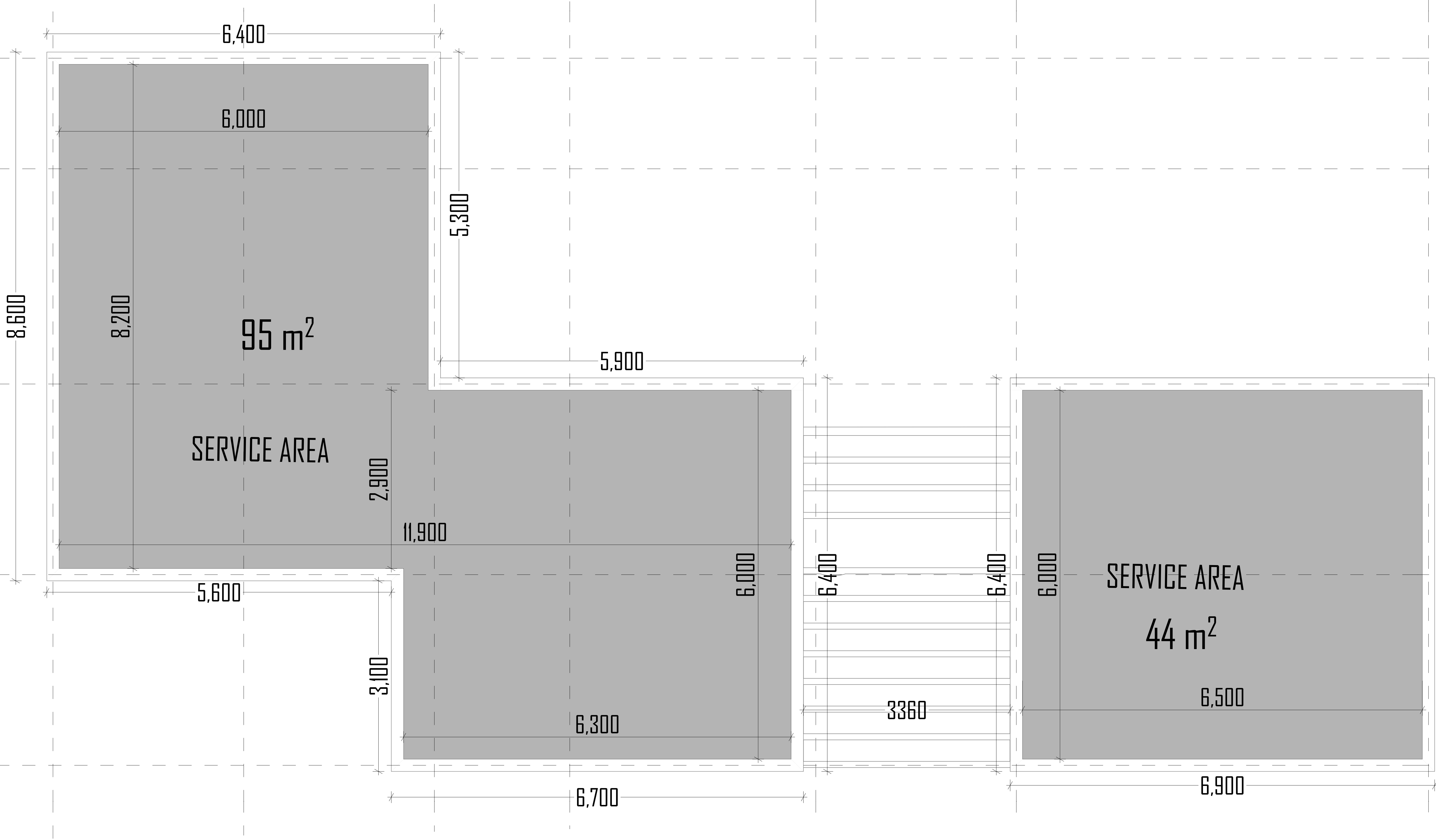
DSQ ROOF PLAN
