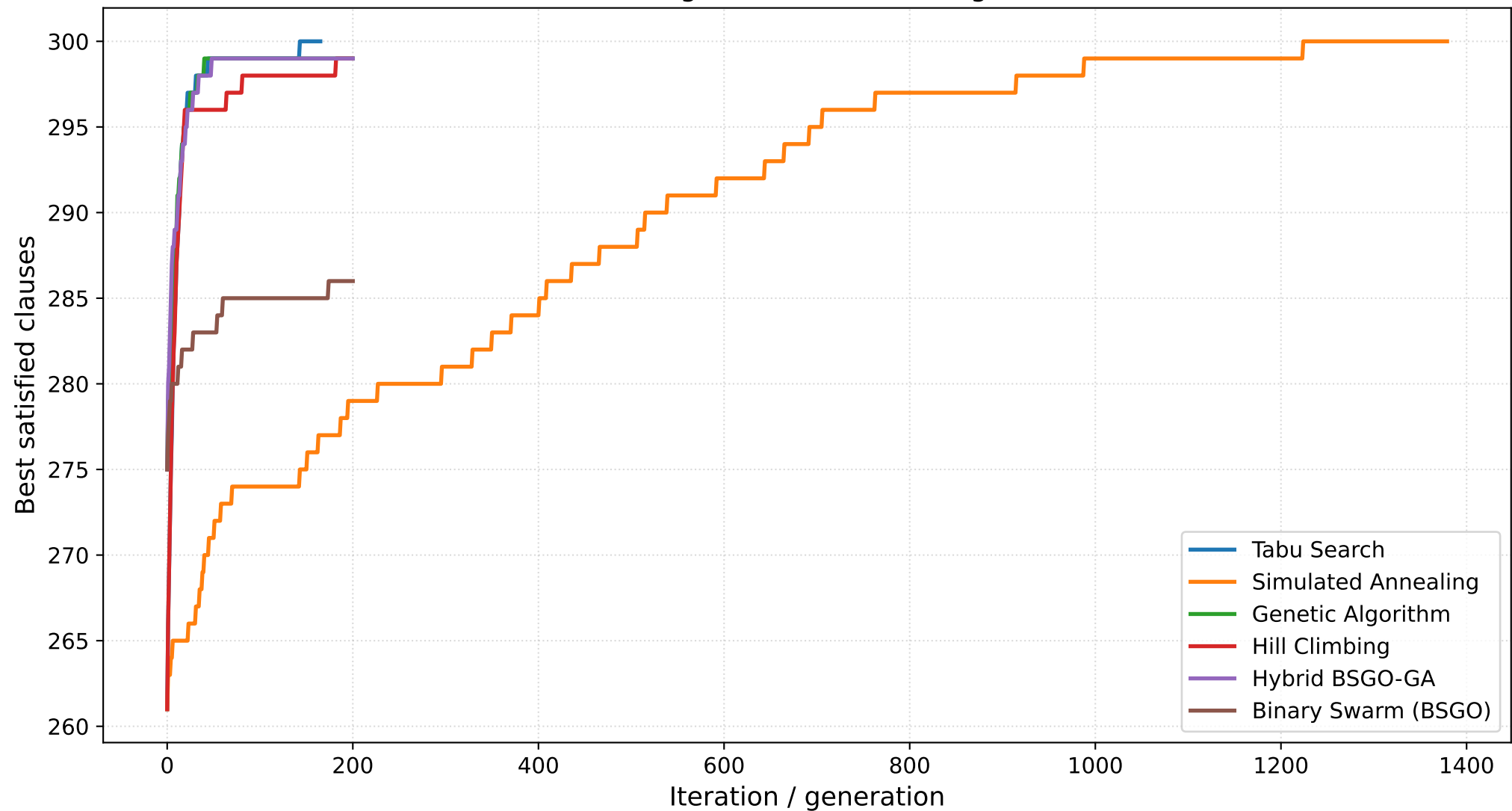
Convergence Curves (Averaged)
