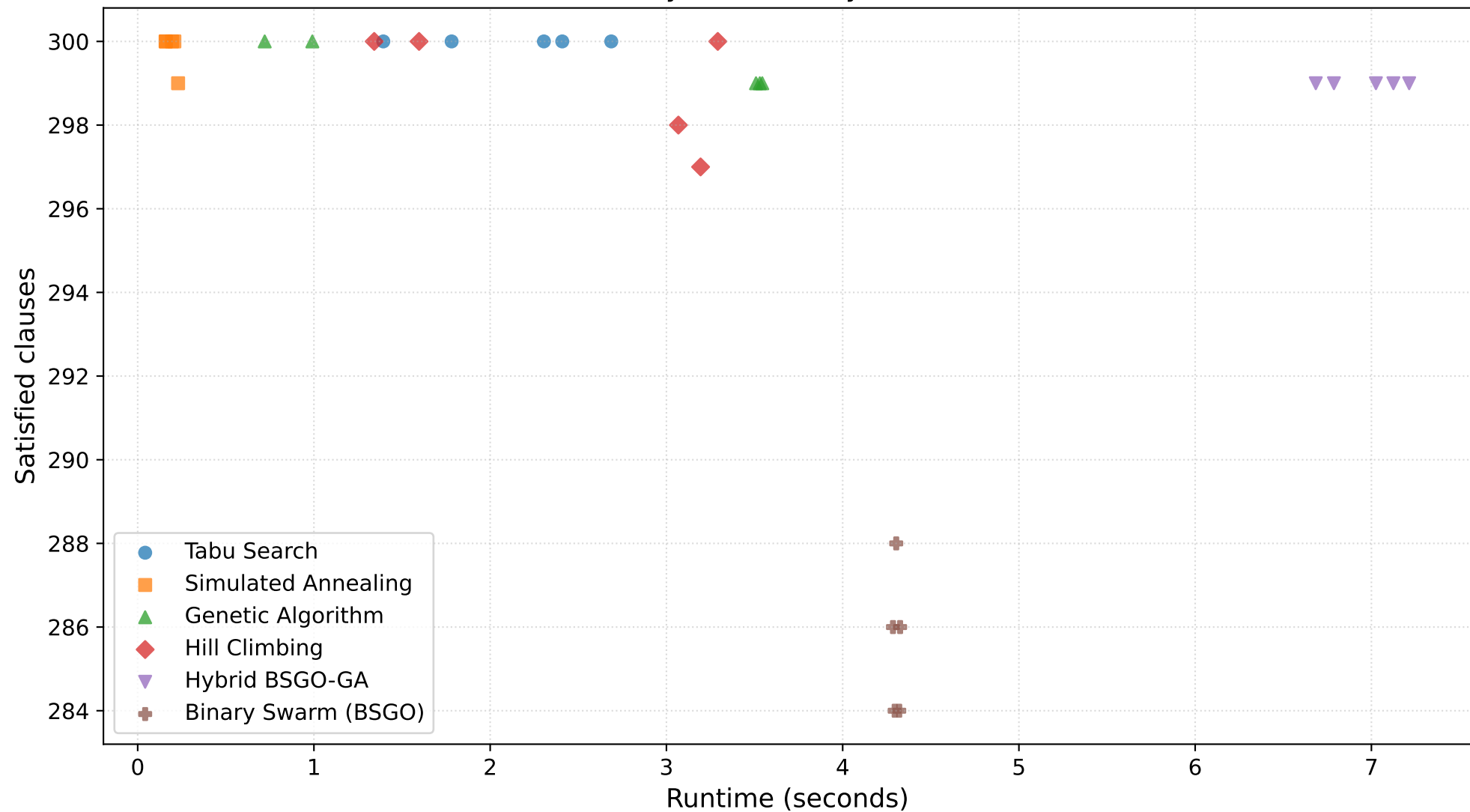
Efficiency Plot: Quality vs Runtime
