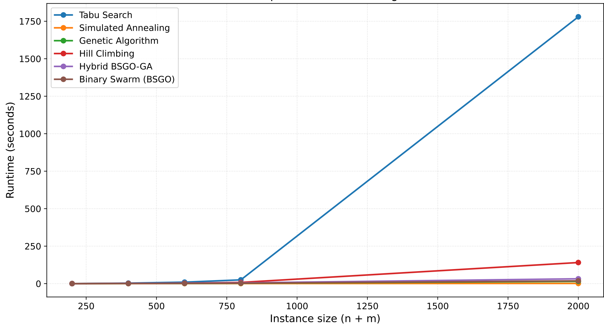
Empirical Runtime Scaling
