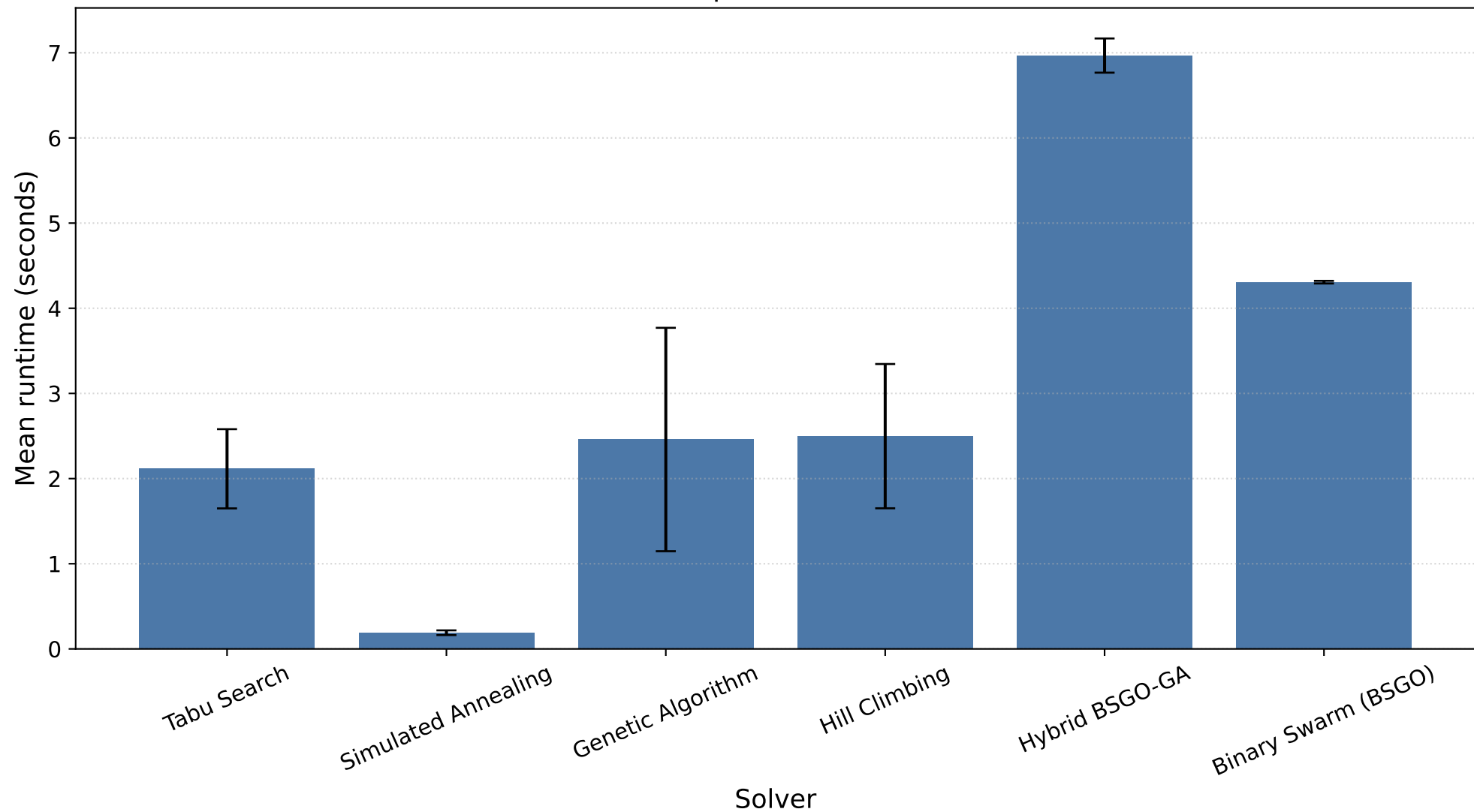
Runtime Comparison Across Solvers
