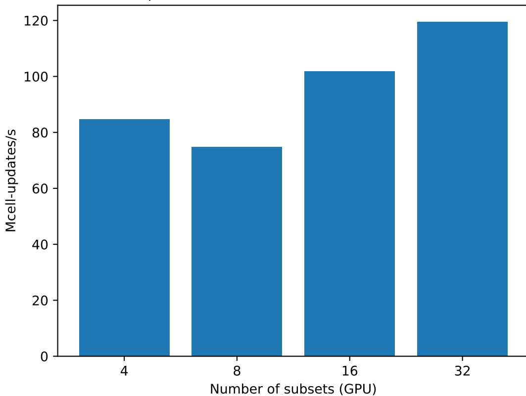
Performance for problem of size 128, with PDI version 1.8.1, on MI250
