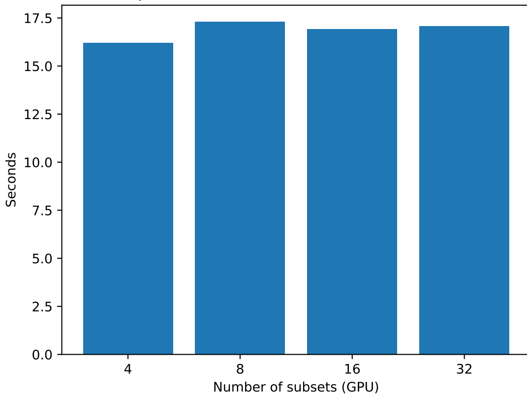
I/O time for problem of size 64, with PDI version 1.8.1, on MI250
