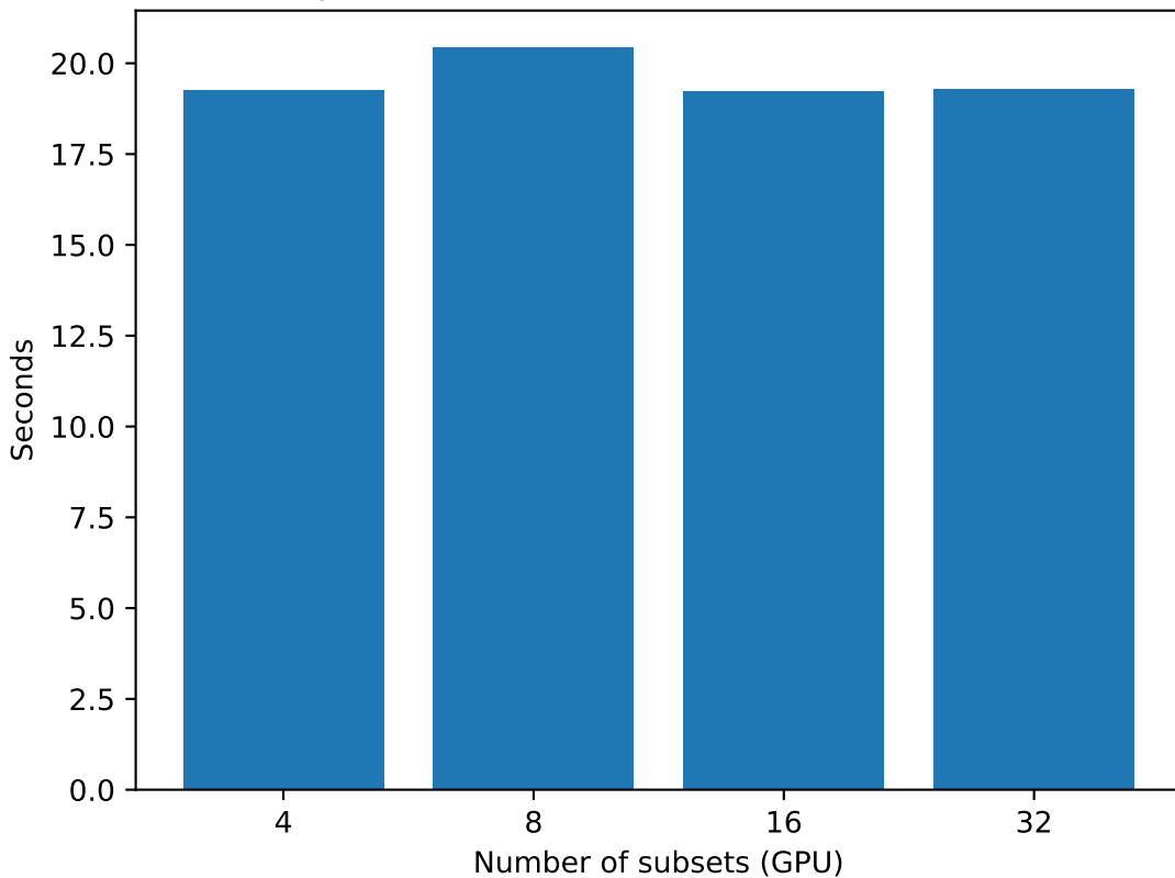
Wall time for problem of size 64, with PDI version 1.8.1, on MI250
