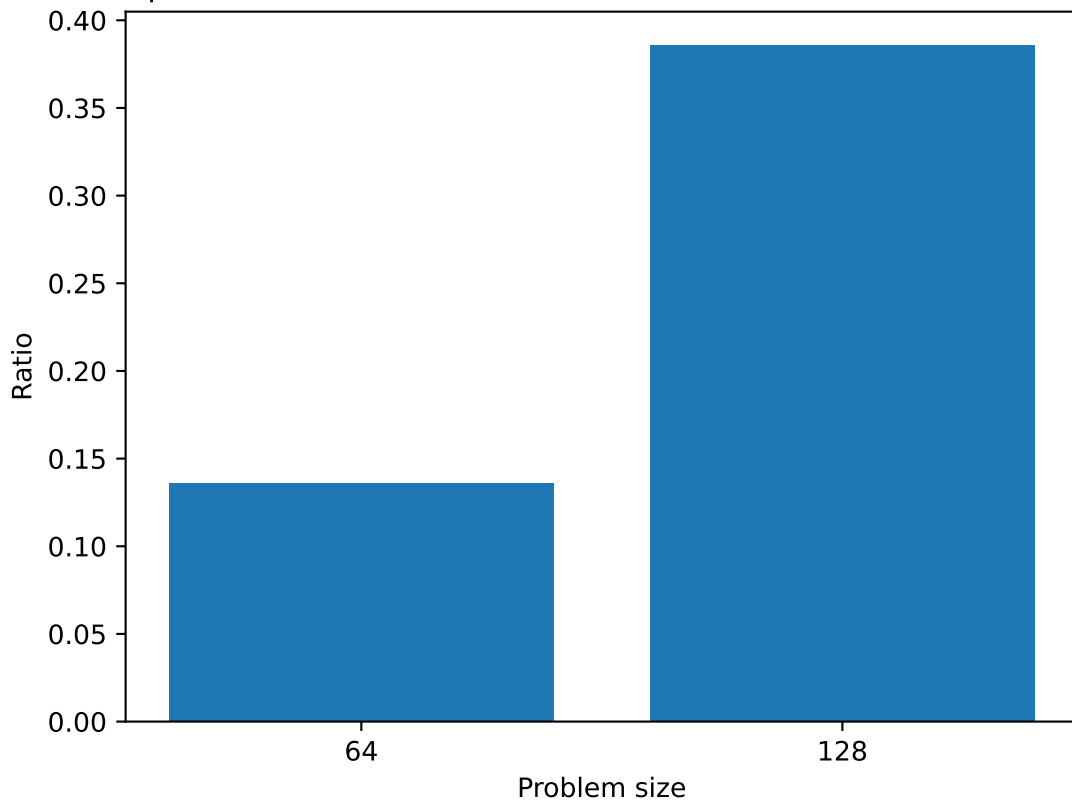
Compute / I/O time with 16 GCD, with PDI version 1.8.1, on MI250
