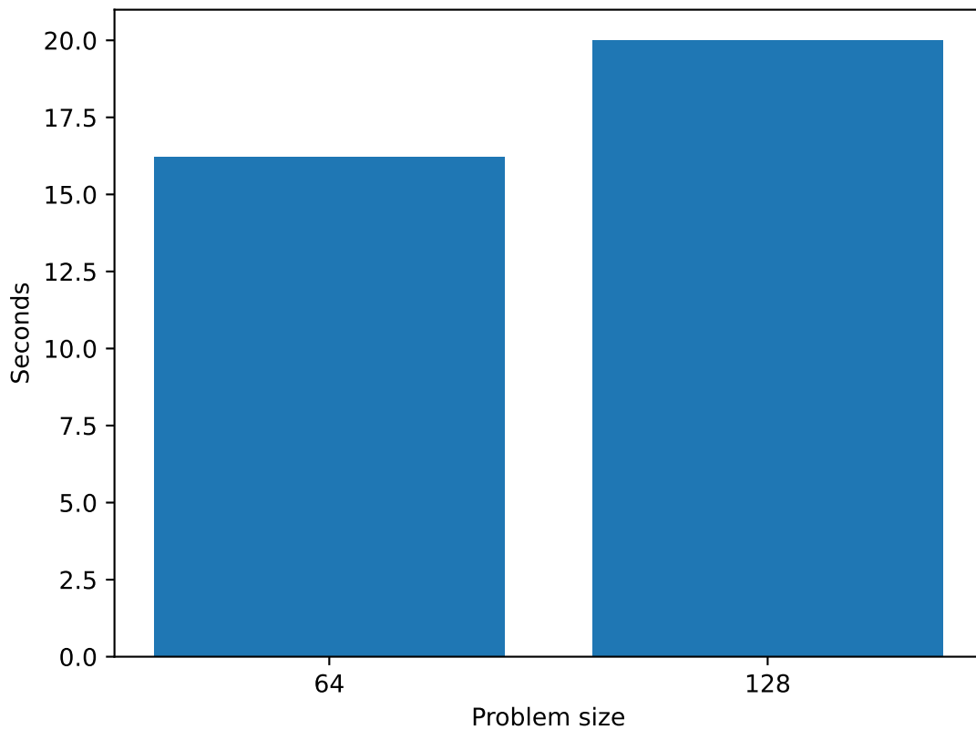
I/O time with 4 GCD, with PDI version 1.8.1, on MI250
