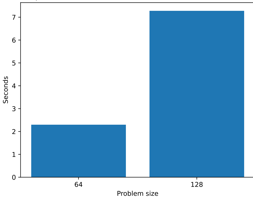
Compute time with 16 GCD, with PDI version 1.8.1, on MI250
