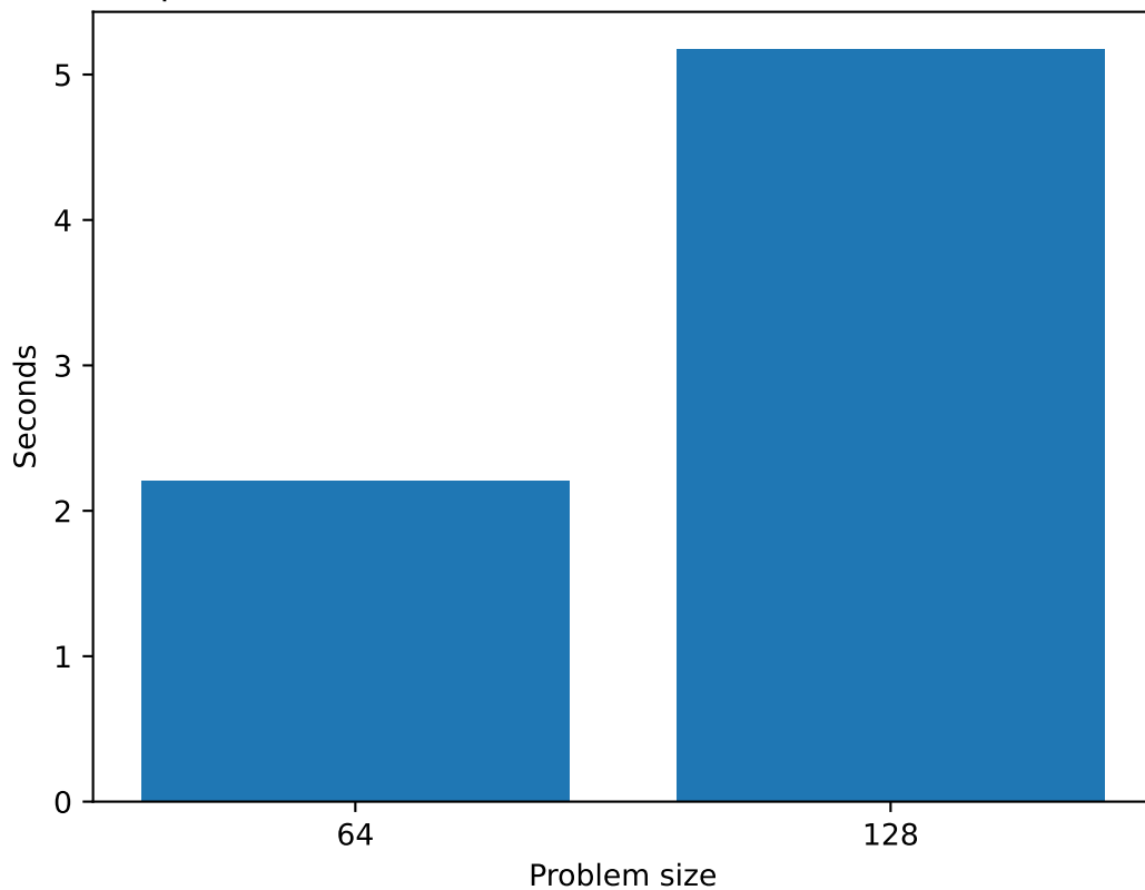
Compute time with 32 GCD, with PDI version 1.8.1, on MI250
