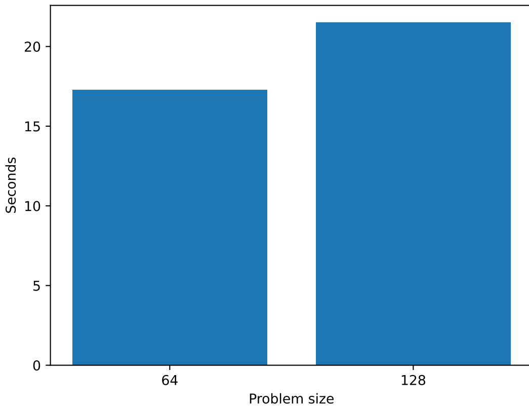
I/O time with 8 GCD, with PDI version 1.8.1, on MI250
