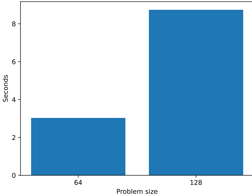
Compute time with 4 GCD, with PDI version 1.8.1, on MI250
