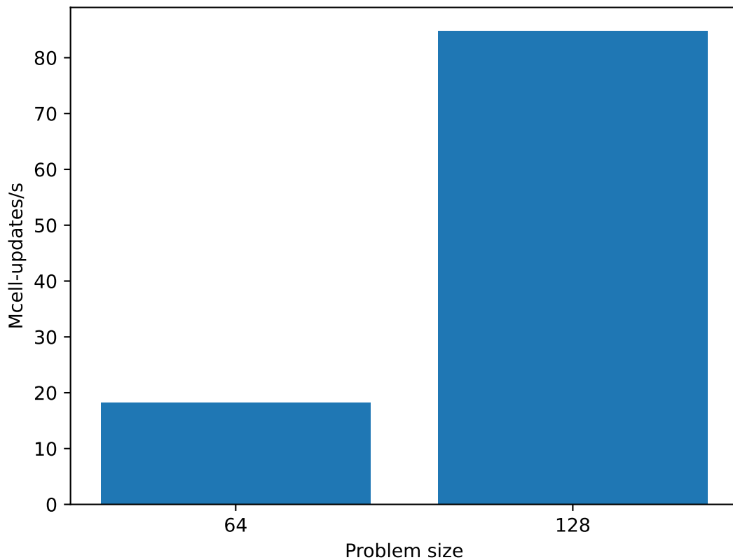
Performance with 4 GCD, with PDI version 1.8.1, on MI250
