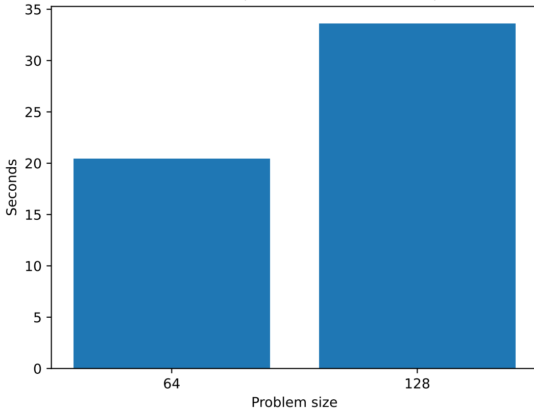
Wall time with 8 GCD, with PDI version 1.8.1, on MI250
