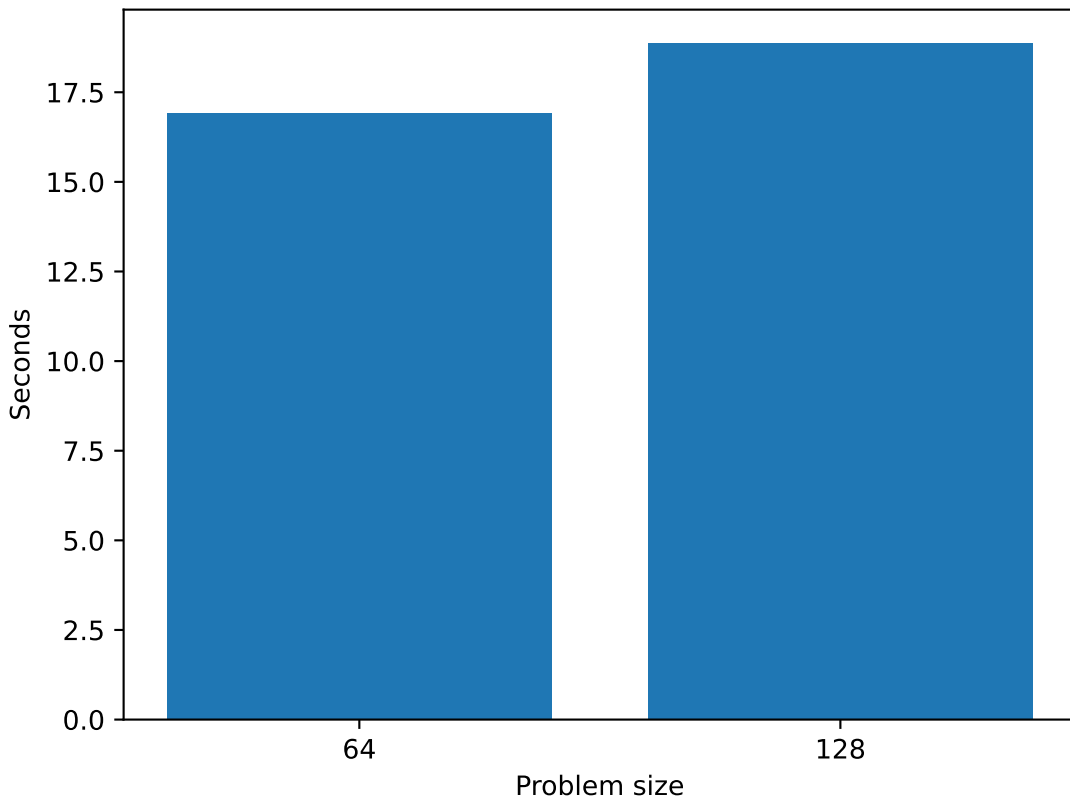
I/O time with 16 GCD, with PDI version 1.8.1, on MI250
