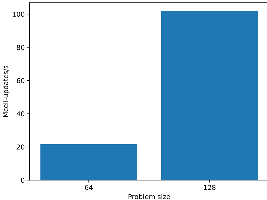
Performance with 16 GCD, with PDI version 1.8.1, on MI250
