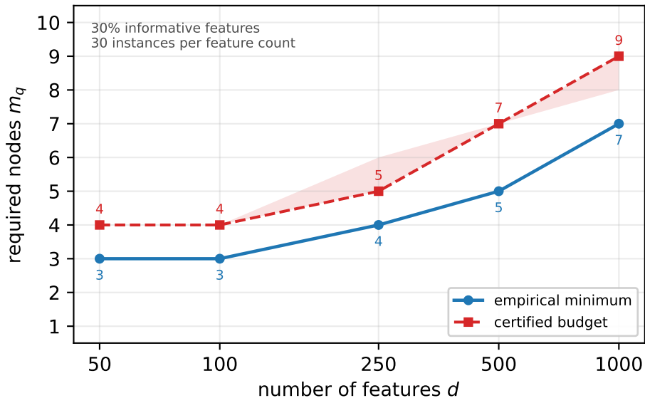
Node growth for absolute error target \varepsilon = 10^{-6}
