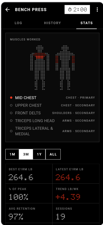
Stats
