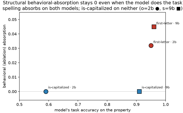
Figure 3: The structural (blue) behavioral-absorption zero persists even as the model’s task accuracy rises from 0.59 to 0.91, while spelling (red) absorbs on both models—so the zero is not a task-performance artifact.
