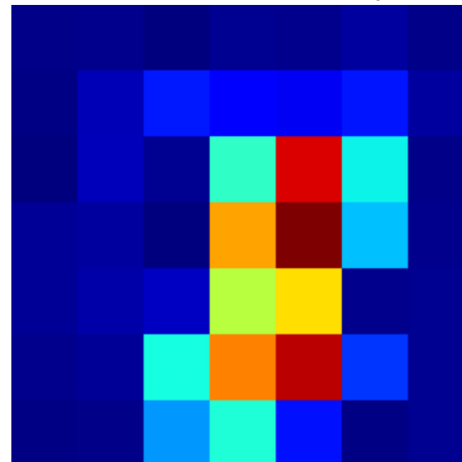
Grad-CAM Heatmap
