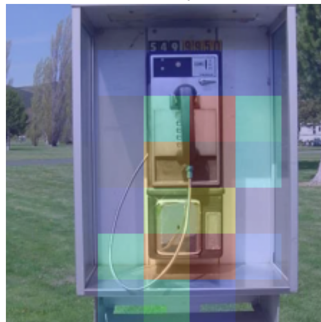
Grad-CAM Explanation
