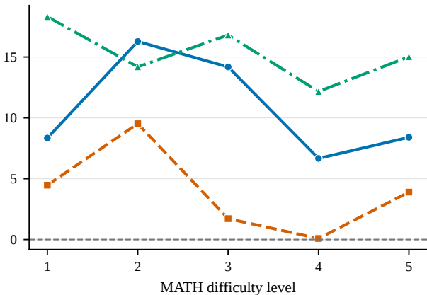
Raw MLP AUROC – judge AUROC (percentage points)
