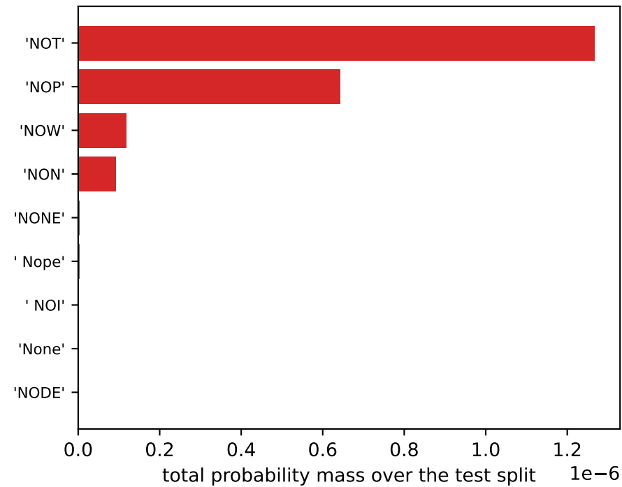
mass the prefix rule counts as NO that is not a NO token
