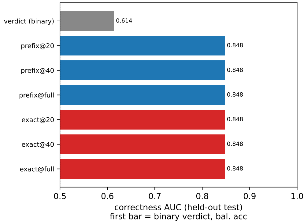
Qwen2.5-7B_MATH: does the binning rule matter?
