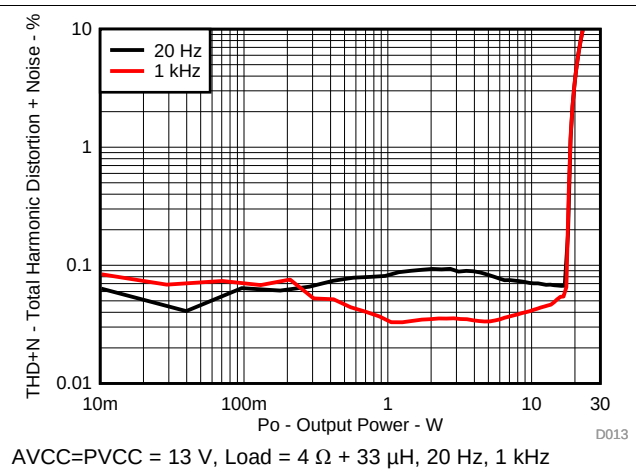
Figure 14. THD+N vs Output Power (PBTL)
