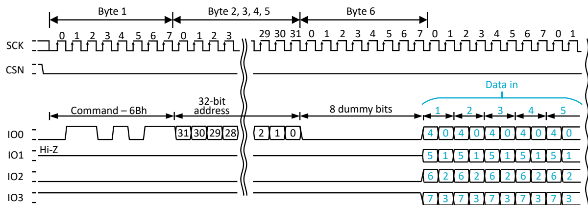
Figure 139: 32-bit READ4O (quad-read output), SPIMODE = MODE0
