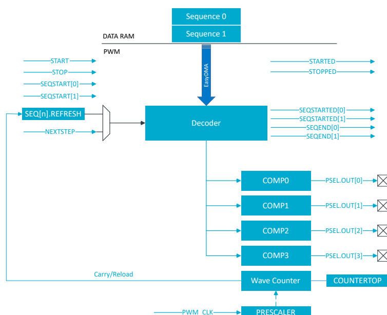
Figure 113: PWM module
