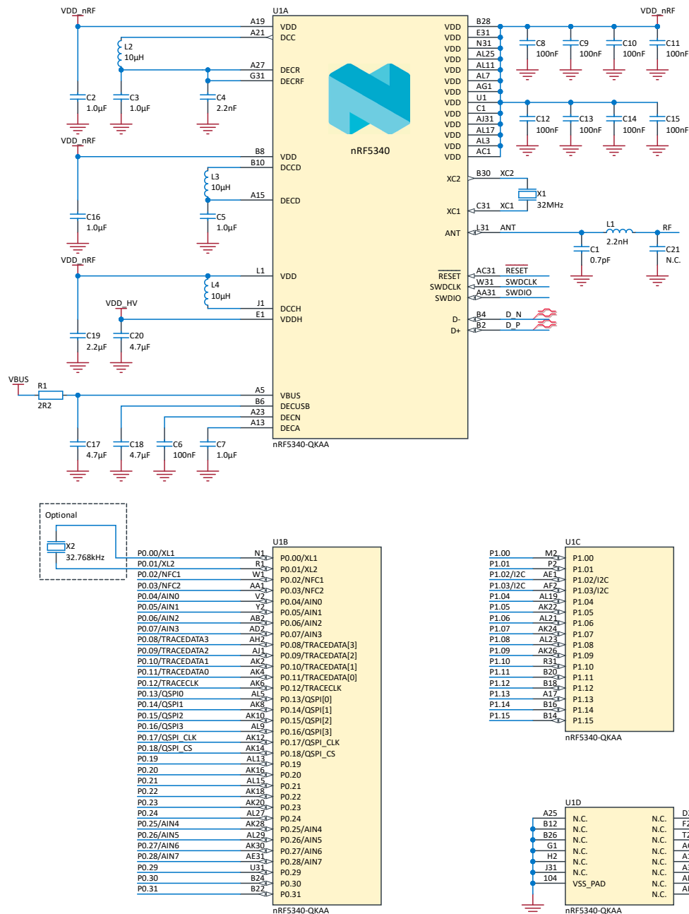
Figure 263: Circuit configuration no. 1 schematic
