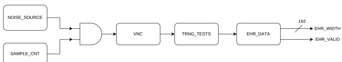
Figure 58: CRYPTOCELL True Random Number Generator
