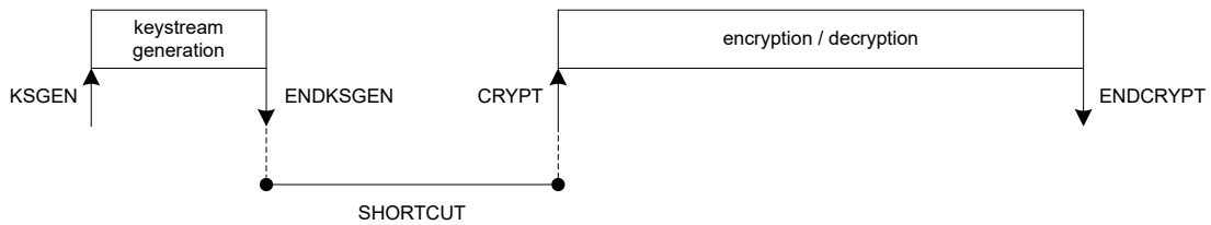
Figure 41: Keystream generation
