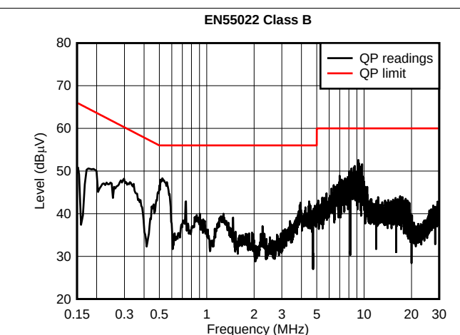
Figure 28. Conducted Emission - Neutral
