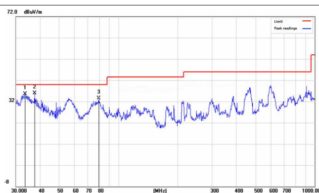
Figure 26. Radiated Emission - Vertical
