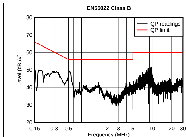
Figure 27. Conducted Emission - Line
