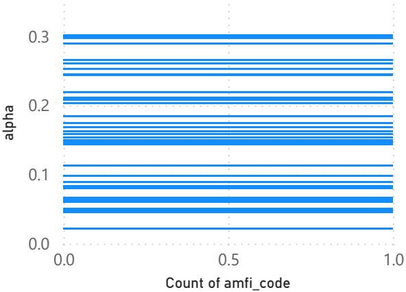
Alpha Ranking
