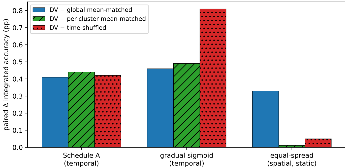
Adaptation-value decomposition (3 seeds, all-paired)
