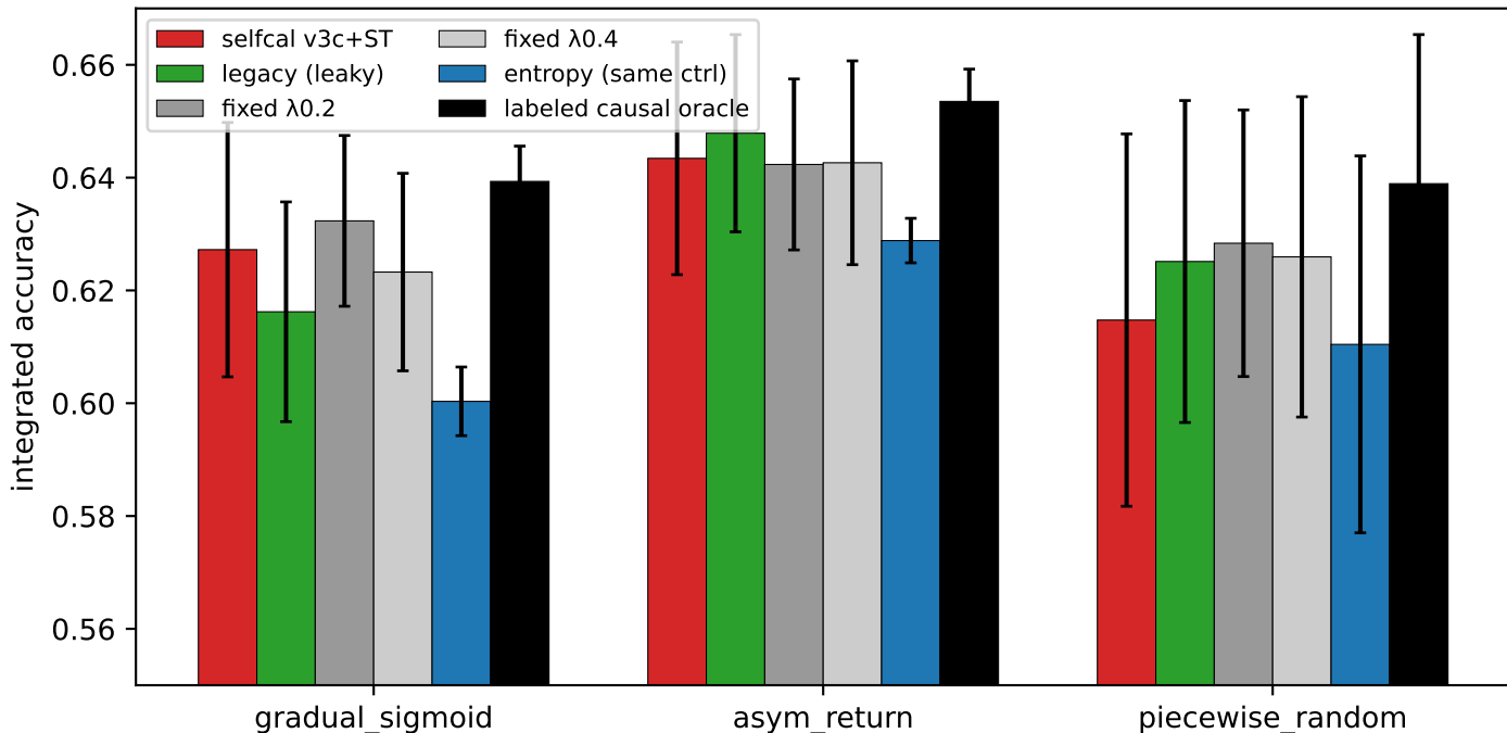
Unseen temporal schedules @150R (5 seeds; ent/oracle 3 seeds)
