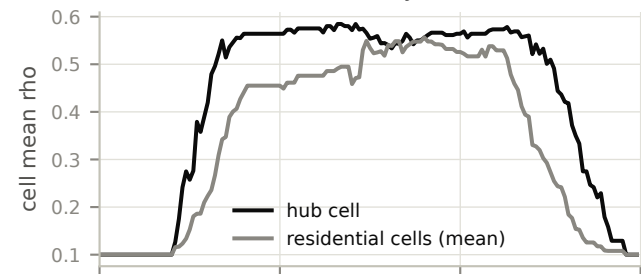
commute mobility (2 seeds)
