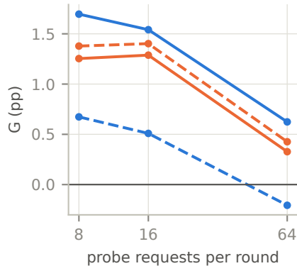
(c) G with probes counted as server use
