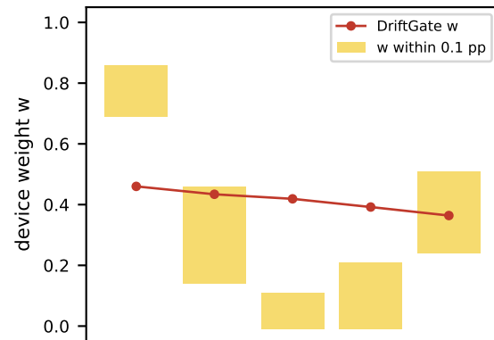
S1, beta 1
