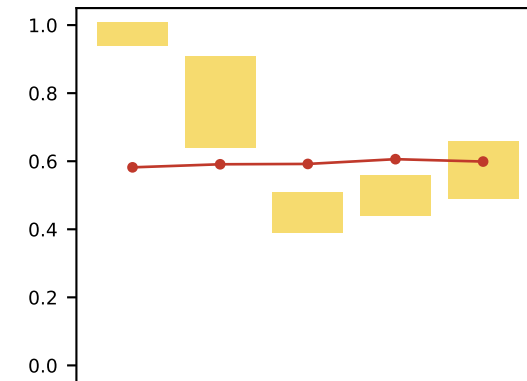
ResNet-18, beta 1
