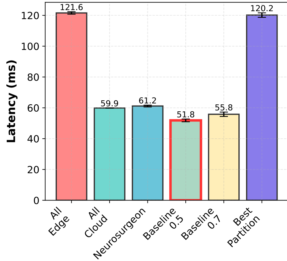
(c) MobileNet-V2
