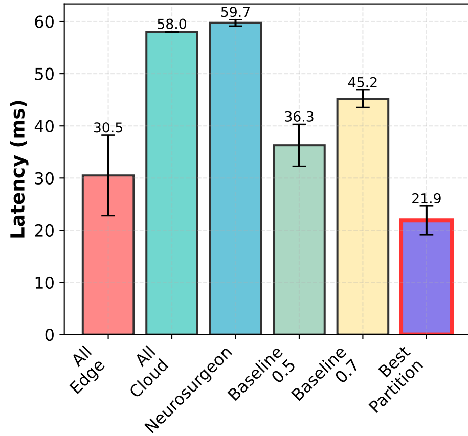
(a) AlexNet
