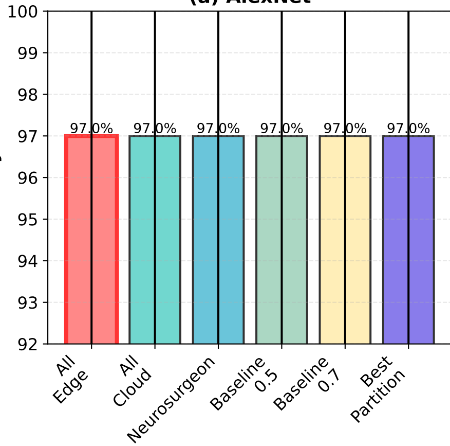
(a) AlexNet
