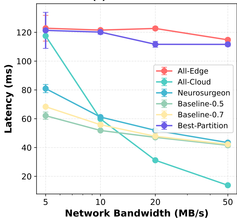
(c) MobileNet-V2
