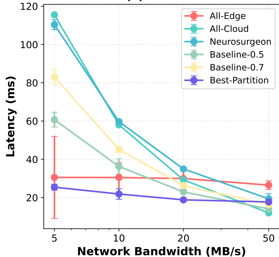
(a) AlexNet
