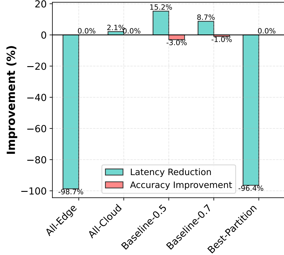
(c) MobileNet-V2 vs Neurosurgeon
