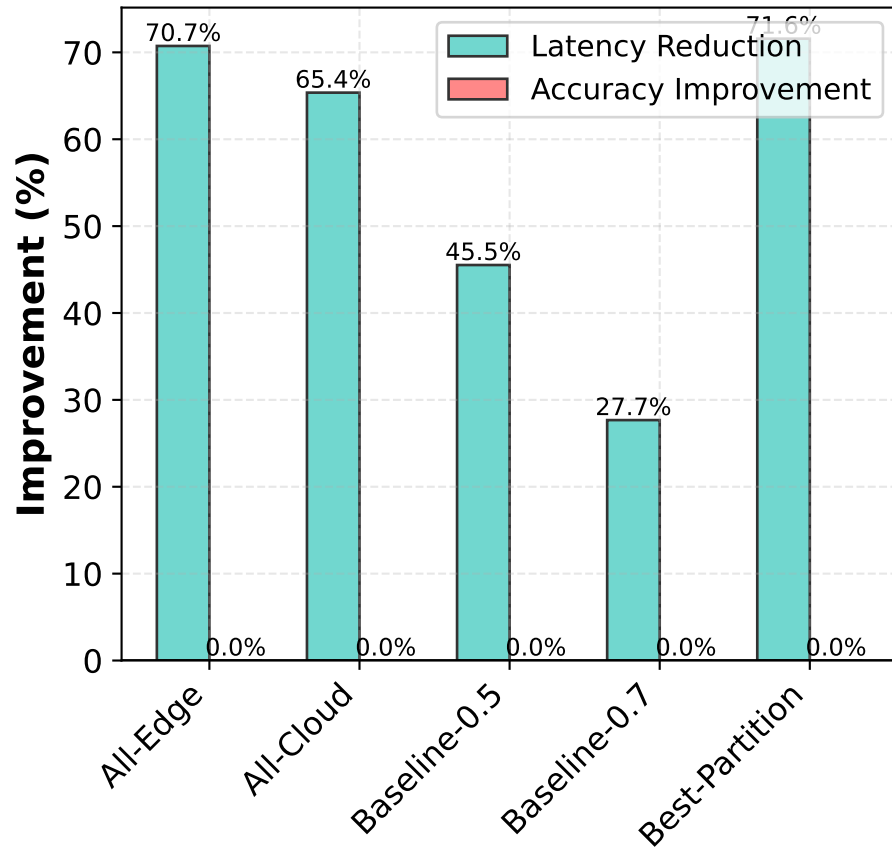
(b) VGG-11 vs Neurosurgeon
