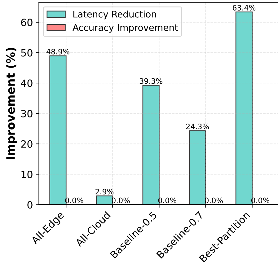
(a) AlexNet vs Neurosurgeon
