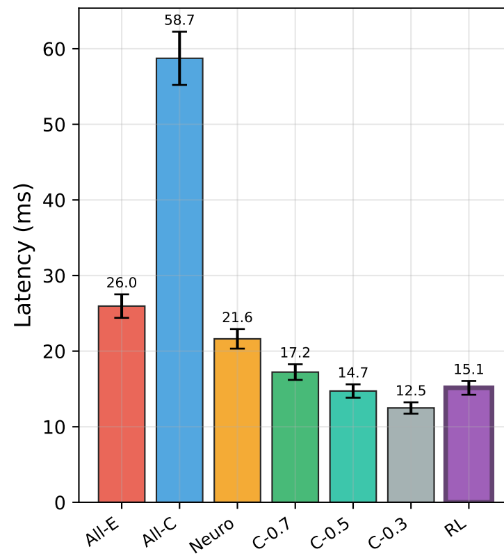
AlexNet
