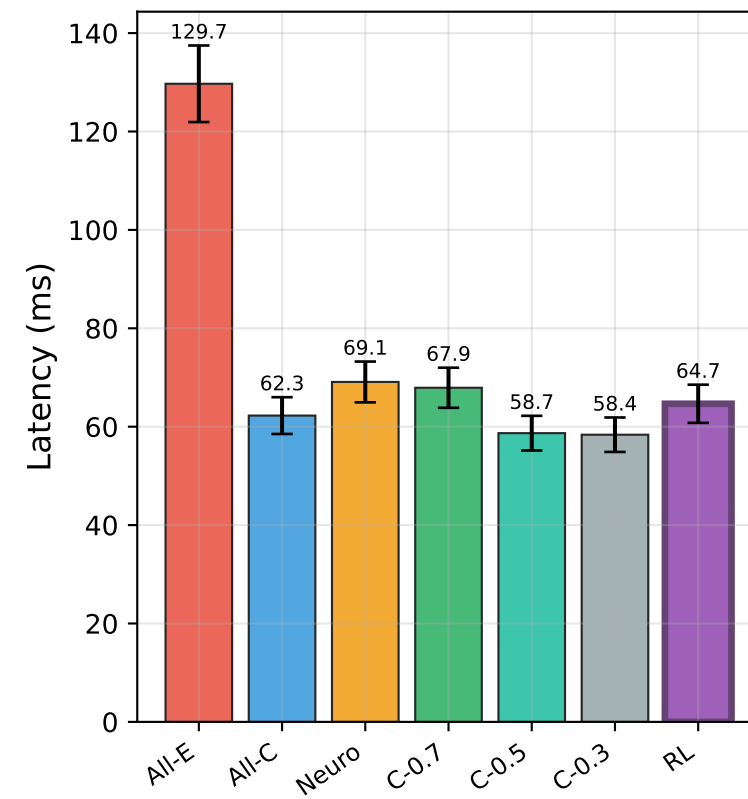
ResNet-50
