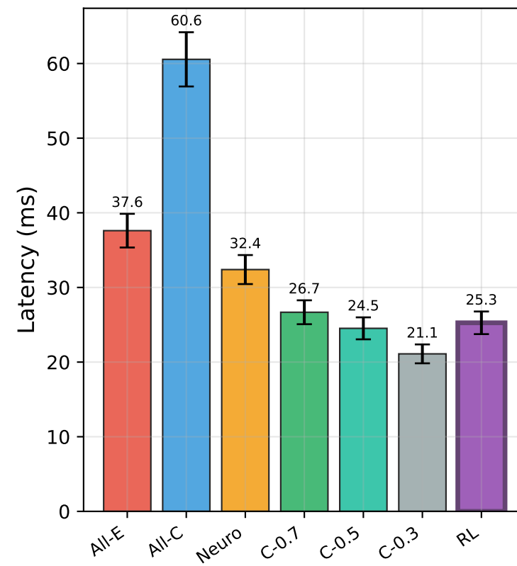
ResNet-18
