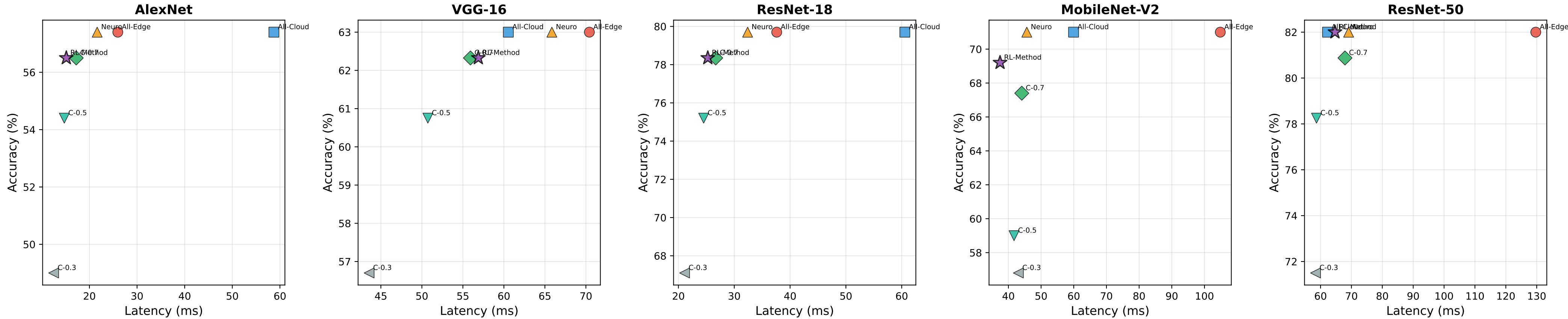
Accuracy-Latency Trade-off (10 MB/s)
