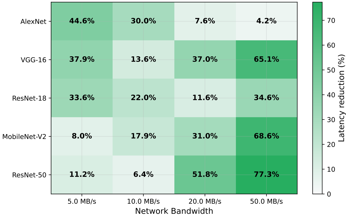
RL-Method Latency Reduction vs. Neurosurgeon (%)
