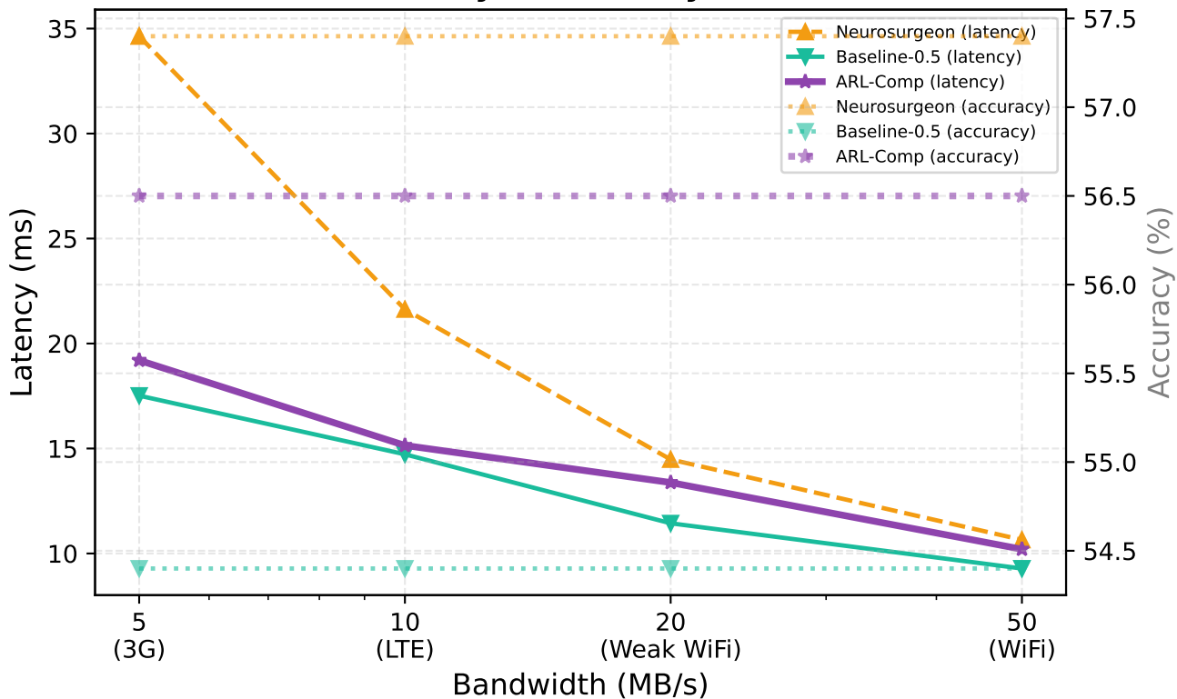
AlexNet: Latency & Accuracy vs. Bandwidth
