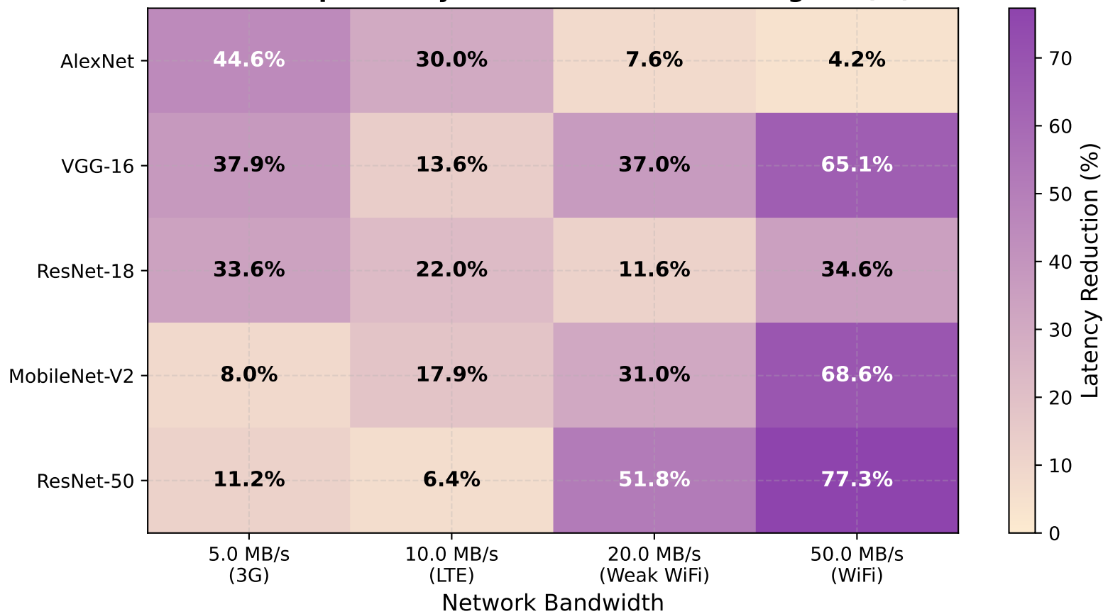
ARL-Comp Latency Reduction vs. Neurosurgeon (%)
